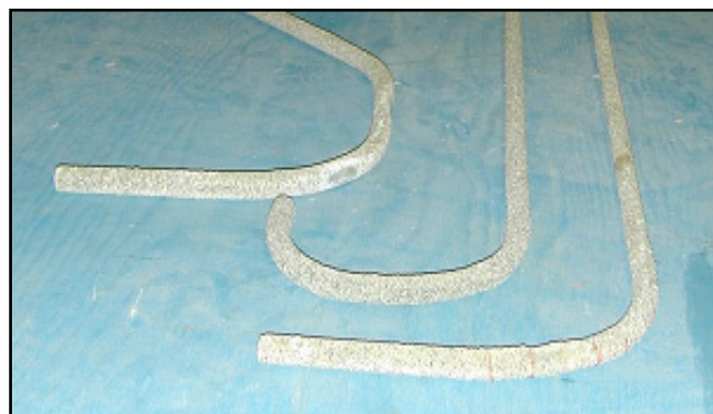
Figure 11.7: Bends in Glass FRP rebar for concrete barrier wall reinforcement (courtesy Vector Construction Group).
